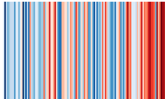
Annual average temperatures for Norway from 1901-2018 using data from Berkeley Earth.
